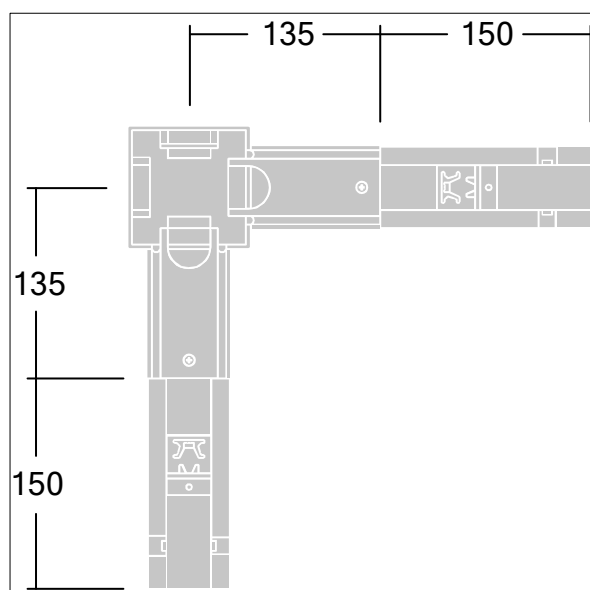
TL_CONTUS_M_L4_Node_Connector.wmf
